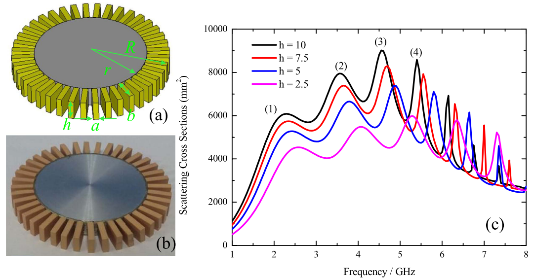
Figure 4. (a) The 3D model of HCGs around a PEC cylindrical core. (b) The fabricated HCGs around an aluminum cylindrical core. (c) The calculated SCSs spectra of the 3D HCGs with \epsilon_{r1} = 20 , \mu_{r1} = 1 around a PEC cylindrical core with different heights ( h = 2.5 mm, 5 mm, 7.5 mm and 10 mm). Peaks (1)–(4) indicate multipolar plasmonic resonances at dipole-, quadru-, hexa-, and octopole modes, respectively.
